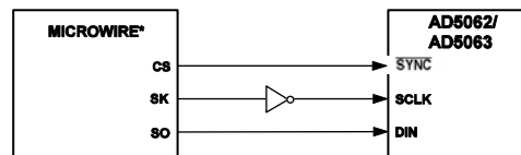
Figure 28. AD5062/AD5063 to MICROWIRE Interface
