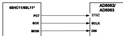
Figure 26. AD5062/AD5063 to 68HC11/68L11 Interface
