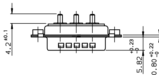
LAYOUT DIMENSIONS (after plating) CONNECTOR SIDE VIEW
