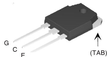
TO-3P (IXSQ)
