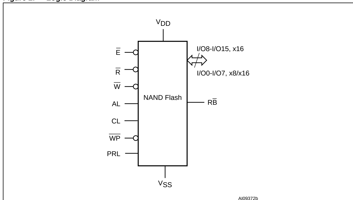
Figure 2. Logic Diagram
