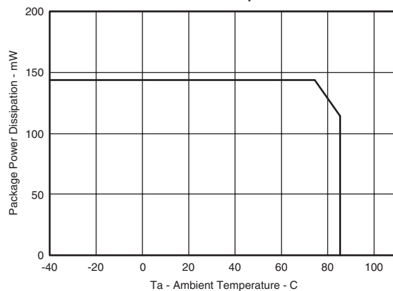
Fig. 21 – Package Power Dissipation vs Ambient Temperature
