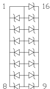
TYPICAL UNI-DIRECTIONAL SCHEMATIC
