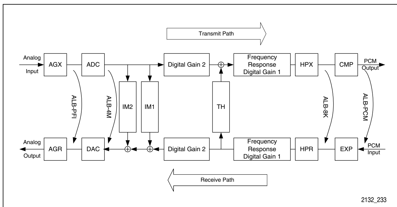
Figure 30 Analog Loops
