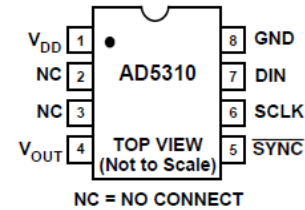
Figure 4. \mu SOIC
