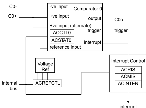
Figure 18-1. Analog Comparator Module Block Diagram
