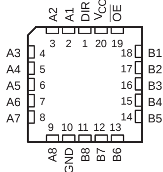
SN54LVTH245A . . . FK PACKAGE (TOP VIEW)
