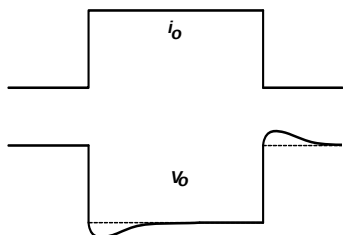
FIGURE 21. LOAD TRANSIENT RESPONSE WHEN C_n IS TOO SMALL
