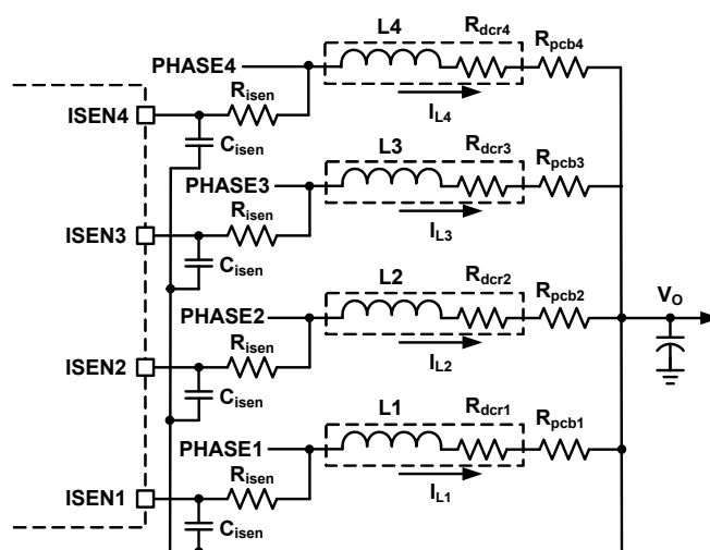
FIGURE 13. CURRENT BALANCING CIRCUIT
