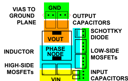
FIGURE 30. TYPICAL POWER COMPONENT PLACEMENT
