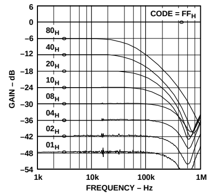
Figure 19. 100 \text{ k}\Omega Gain vs. Frequency vs. Code
