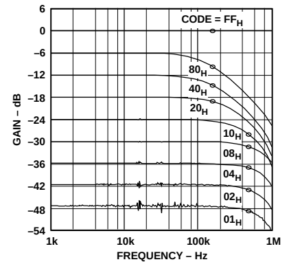
Figure 16. 50 \text{ k}\Omega Gain vs. Frequency vs. Code
