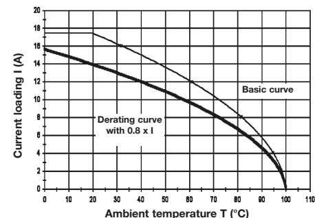
LM3R 5.08/90/6 poles with Conductor H07V-K1.5 mm 2
