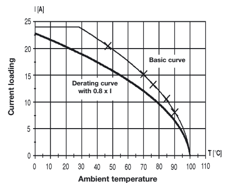
LPZF 5.08/2/180 3.2 OR with Conductor H07V-K2.5 mm 2
