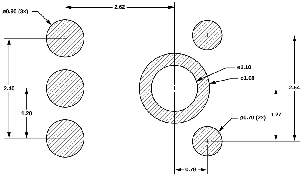
Figure 8. PCB Land Pattern Layout
