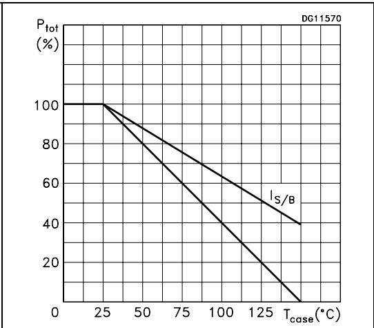
Figure 3. Derating curve
