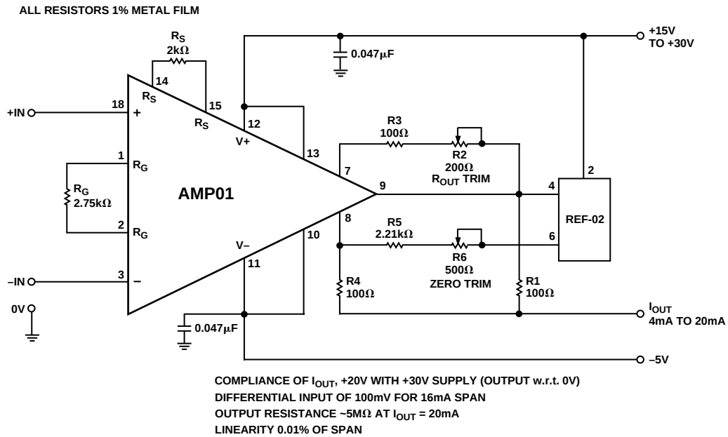
Figure 37. 13-Bit Linear 4–20 mA Transmitter Constructed by Adding a Voltage Reference. Thermocouple Signals Can Be Accepted Without Preamplication.
