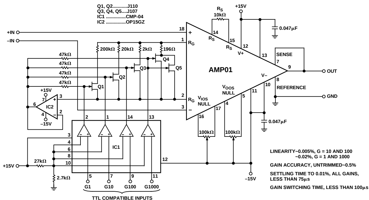
Figure 39. The AMP01 Makes an Excellent Programmable-Gain Instrumentation Amplifier. Combined Gain-Switching and Settling Time to 13 Bits Falls Below 100\mu\text{s} . Linearity Is Better than 12 Bits over a Gain Range 1 to 1000.
