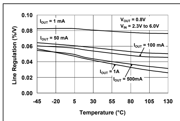
FIGURE 2-15: Line Regulation vs. Temperature.
