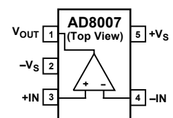
Figure 2. 5-Lead SC70 (KS)
