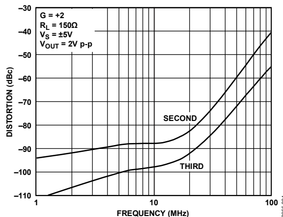
Figure 4. AD8007 Second and Third Harmonic Distortion vs. Frequency
