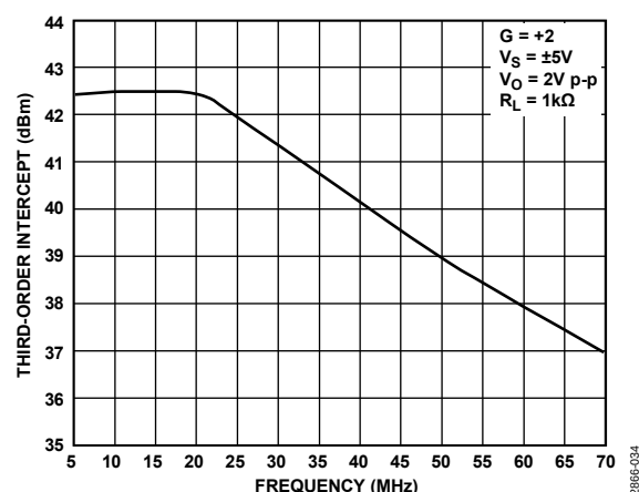
Figure 34. AD8008 Third-Order Intercept vs. Frequency
