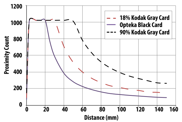
Figure 11a. Proximity Distance Profile (8Pulse, 100 mA, 1×)
