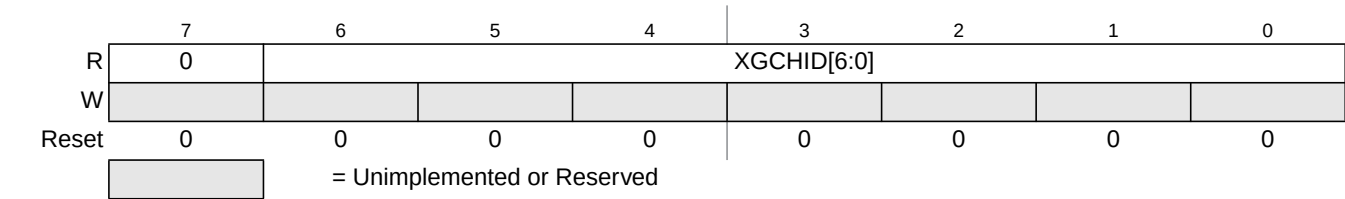
Figure 6-4. XGATE Channel ID Register (XGCHID)
