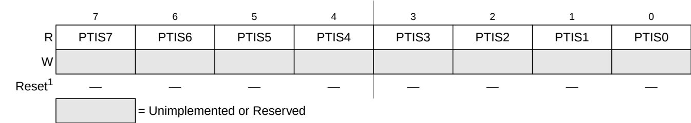
Figure 22-26. Port S Input Register (PTIS)
