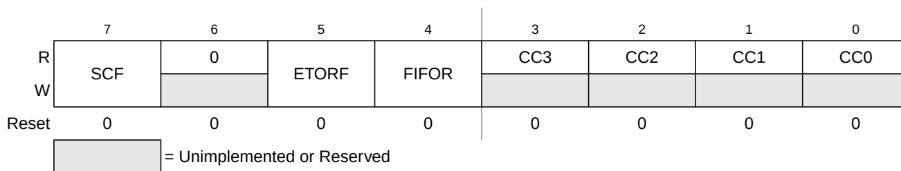
Figure 4-9. ATD Status Register 0 (ATDSTAT0)
