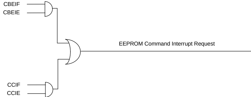
Figure 25-24. EEPROM Interrupt Implementation
