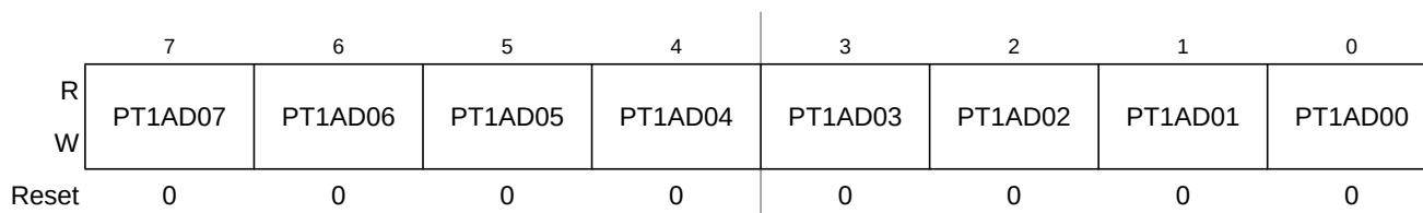
Figure 22-64. Port AD0 Data Register 1 (PT1AD0)
