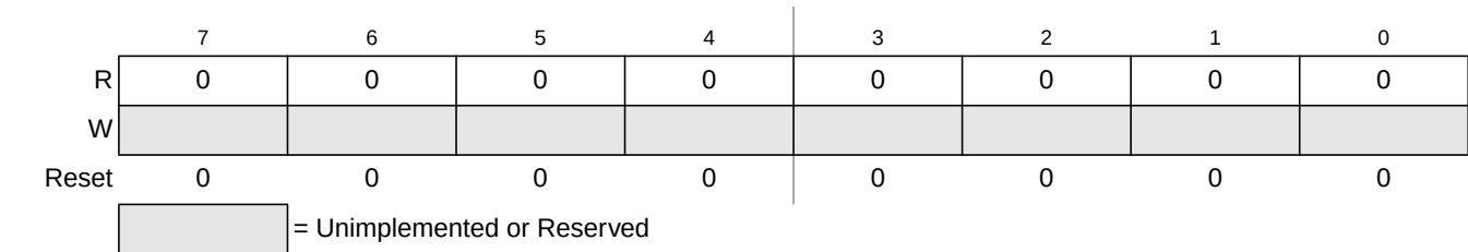
Figure 26-12. RESERVED3
