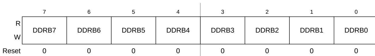
Figure 22-6. Port B Data Direction Register (DDRB)
