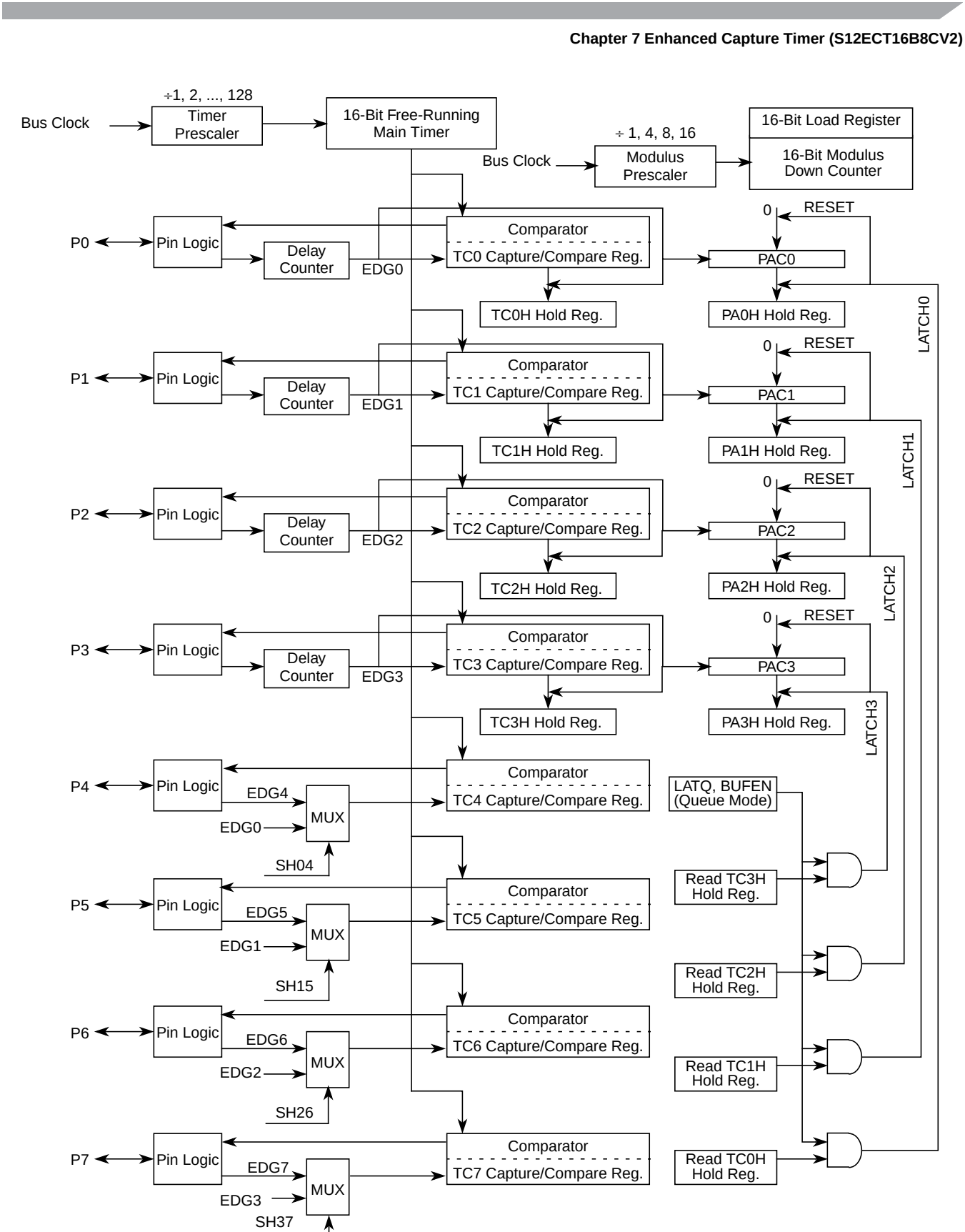
Figure 7-67. Detailed Timer Block Diagram in Queue Mode when PRNT = 0
