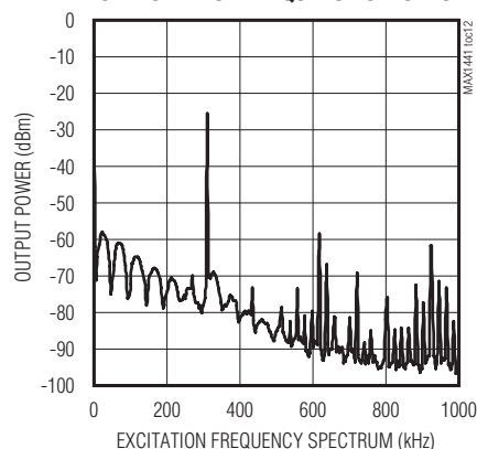
OUTPUT POWER vs. EXCITATION FREQUENCY SPECTRUM
