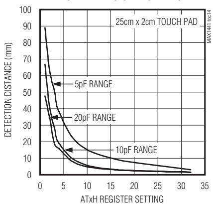
DETECTION DISTANCE vs. ATxH REGISTER SETTING
