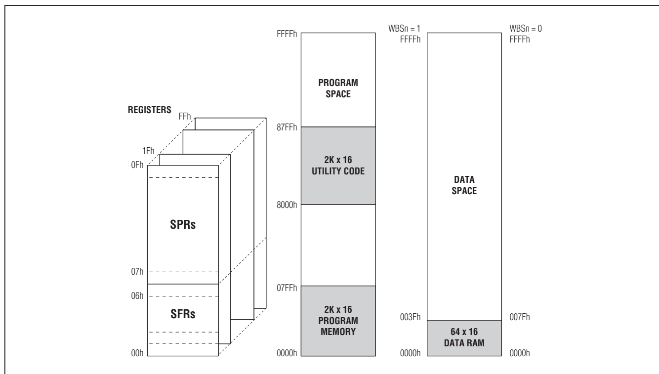
Figure 3. Memory Map
