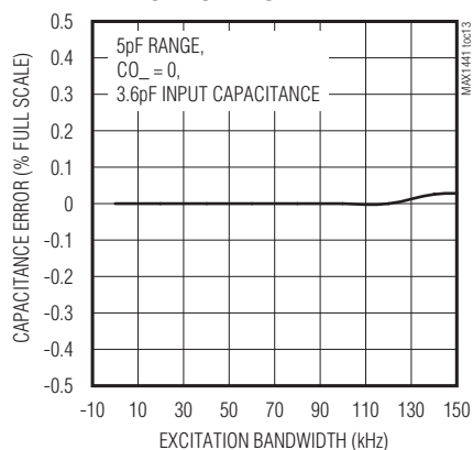
CAPACITANCE ERROR vs. EXCITATION BANDWIDTH
