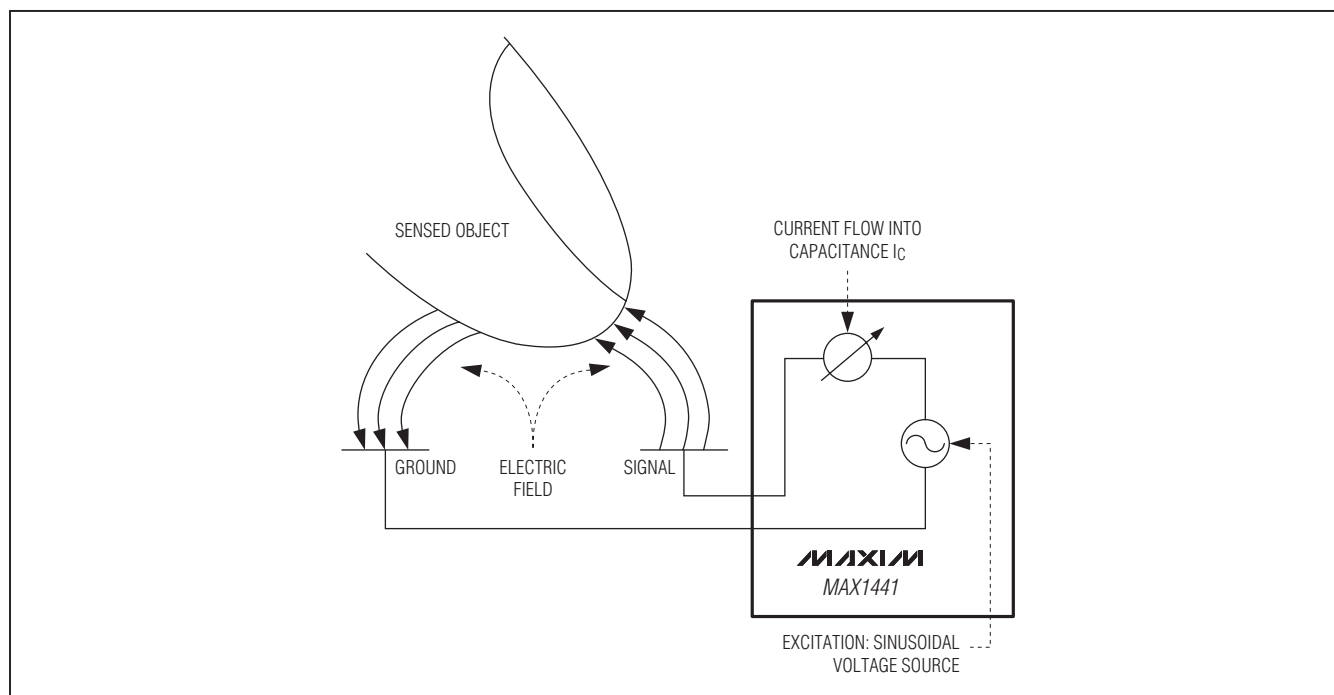
Figure 2. Capacitive-Sensing Function
