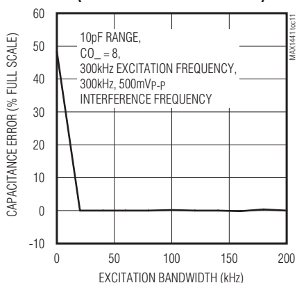
CAPACITANCE ERROR vs. EXCITATION BANDWIDTH (WITH IN-BAND INTERFERENCE)
