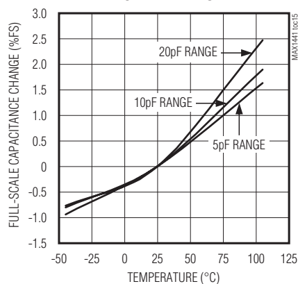
FULL-SCALE CAPACITANCE CHANGE vs. TEMPERATURE
