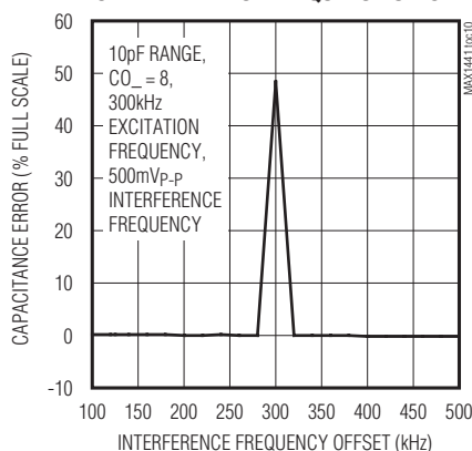
CAPACITANCE ERROR vs. INTERFERENCE FREQUENCY OFFSET
