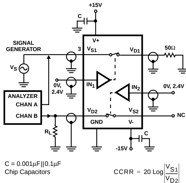
FIGURE 4. CHANNEL TO CHANNEL CROSSTALK TEST CIRCUIT
