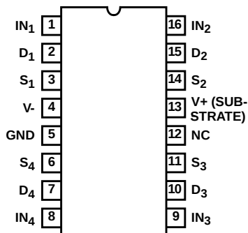
DG201A, DG202 (CERDIP, PDIP, SOIC) TOP VIEW
