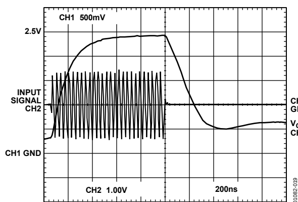
Figure 19. Large Signal Response Time
