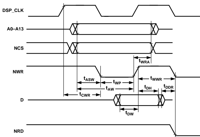
Figure 6. Write Operation
