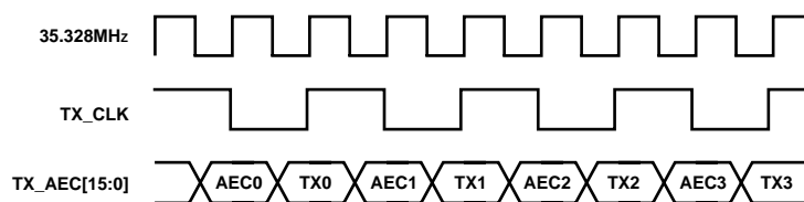
Figure 11. TX_AEC Mux Bus in Normal Operation
