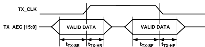
Figure 1. TX Timing
