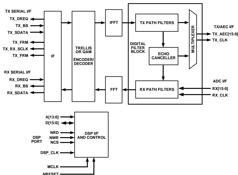
Figure 8. Block Diagram
