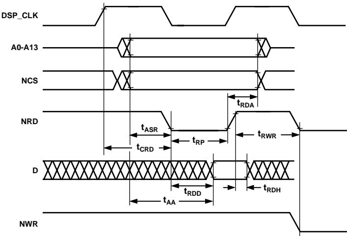
Figure 5. Read Operation
