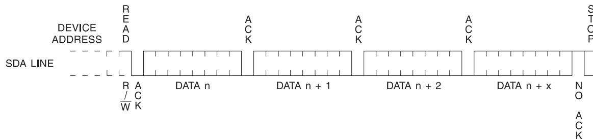
Figure 9. Sequential Read
