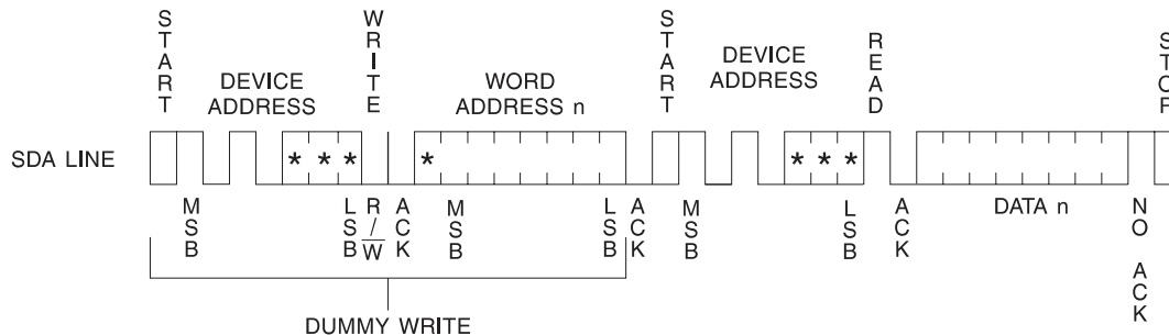
Figure 8. Random Read
