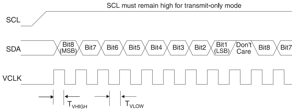
Figure 1. Transmit-only Mode
