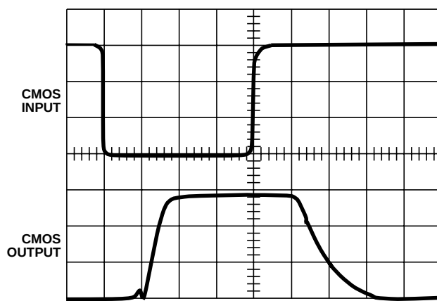
FIGURE 6. LOGIC "0" = SWITCH ON
