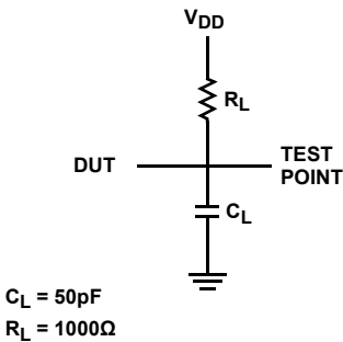
FIGURE 5. THREE-STATE LOW LOAD CIRCUIT
