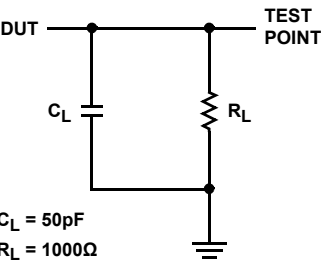
FIGURE 6. THREE-STATE HIGH LOAD CIRCUIT
