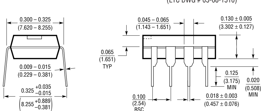
N8 Package 8-Lead PDIP (Narrow 0.300) (LTC DWG # 05-08-1510)
