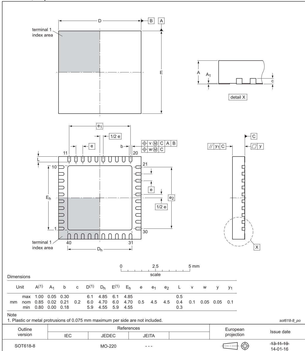
Fig 52. Package outline SOT618-8 HVQFN40
