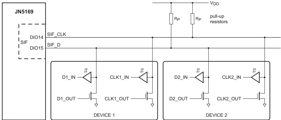
Fig 35. Connection details
