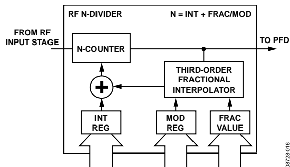
Figure 18. RF N-Divider
