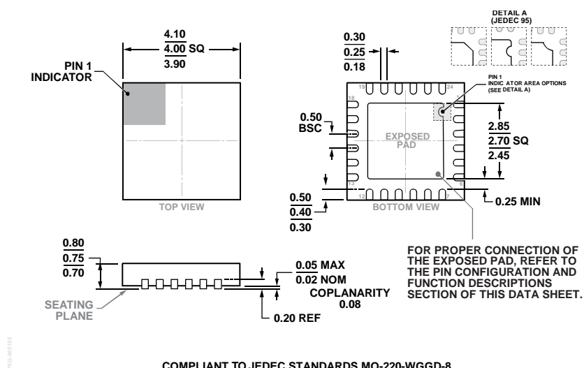
Figure 49. 24-Lead Lead Frame Chip Scale Package [LFCSP] 4 mm × 4 mm Body and 0.75 mm Package Height (CP-24-8)
