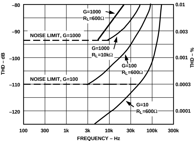
Figure 42. Total Harmonic Distortion (THD) vs. Frequency @ 3 V rms for Figure 41b
