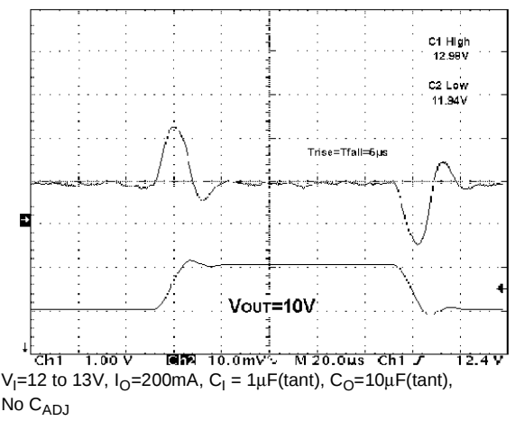
Figure 26: Line Transient
