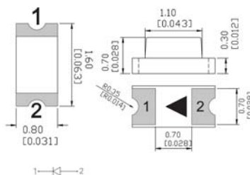
Package Outline Drawing:
