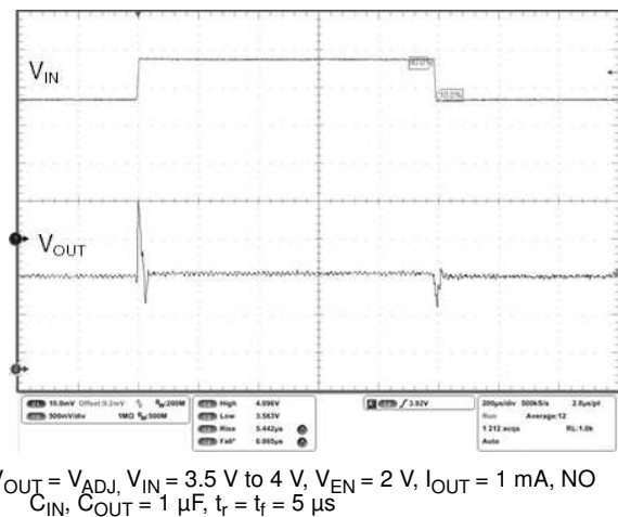
Figure 26. Line transient ( V_{OUT} = V_{ADJ} )
