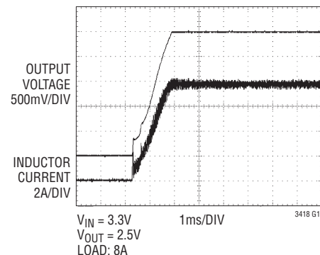
Start-Up Transient
