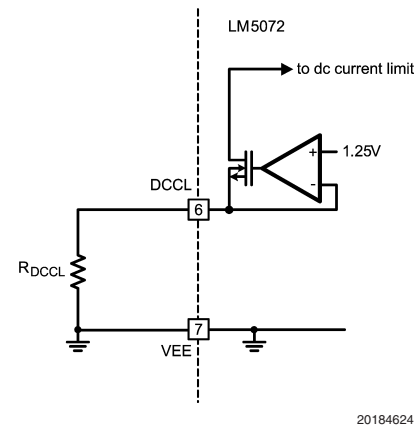
FIGURE 8. Input DC Current Limit Programming via R_{DCCCL}
