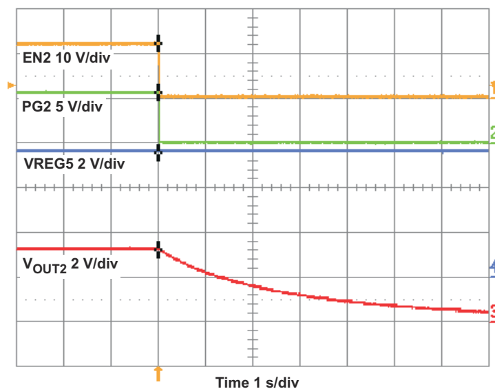
Figure 4-23. TPS54294EVM Shut-Down Relative to EN2
