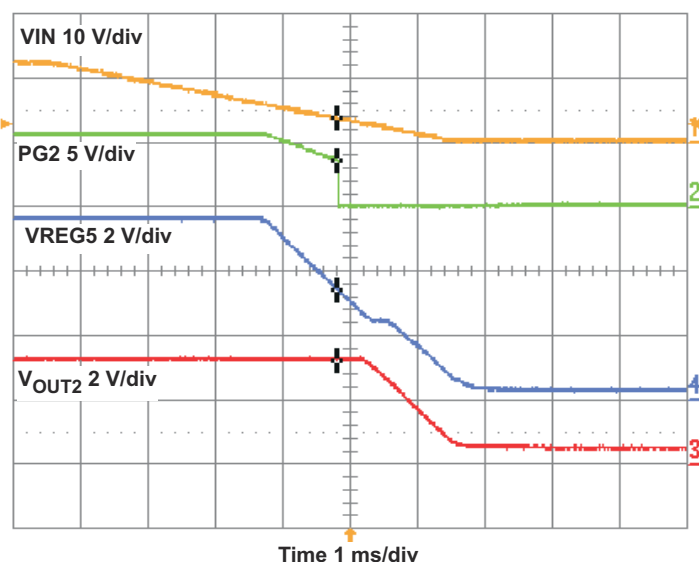
Figure 4-21. TPS54294EVM Converter 2 Shut-Down Relative to V_{IN}
