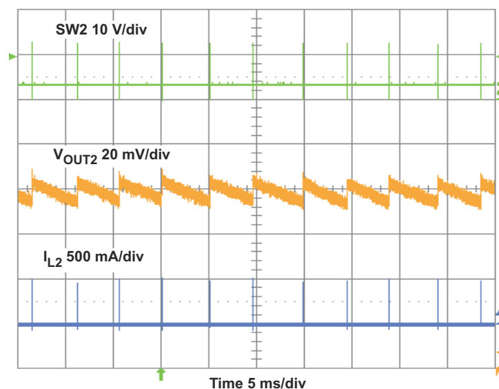
Figure 4-14. TPS54294EVM Converter 2 Eco-mode™ Output Voltage Ripple at No Load
