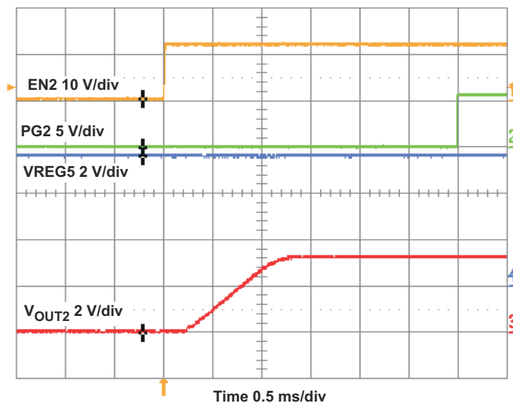
Figure 4-22. TPS54294EVM Start-Up Relative to EN2
