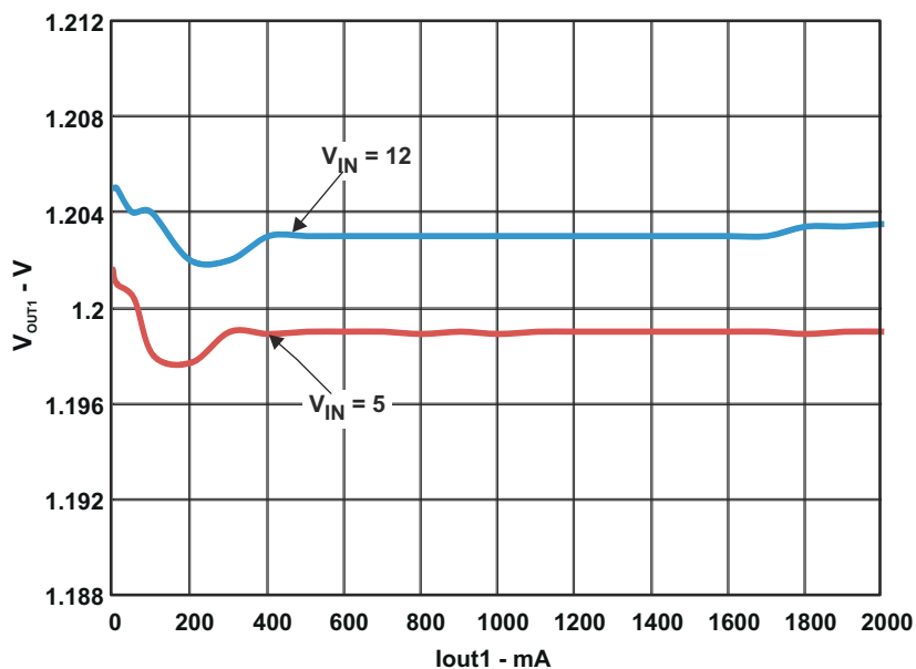
Figure 4-3. TPS54294EVM Converter 1 Load Regulation
