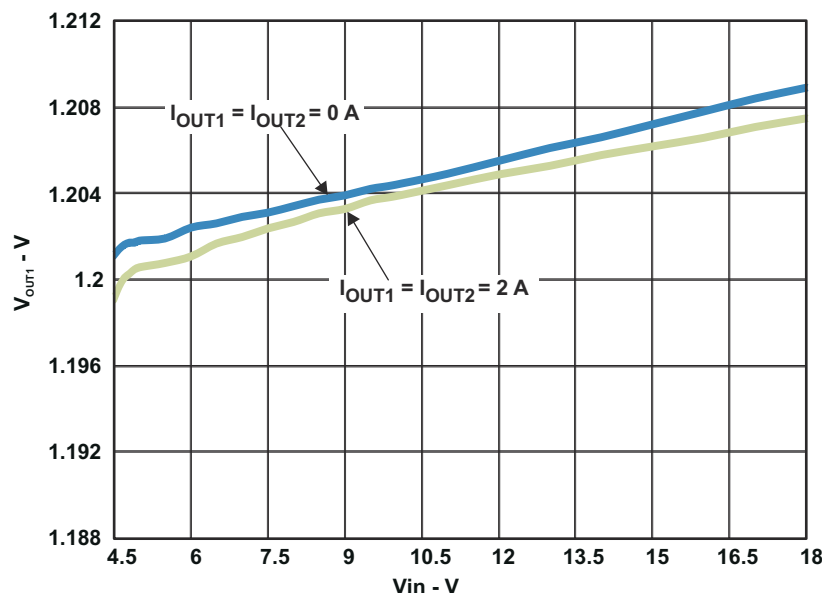
Figure 4-5. TPS54294EVM Converter 1 Line Regulation
