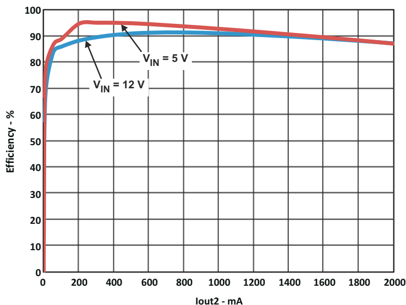
Figure 4-2. TPS54294EVM Converter 2 Efficiency
