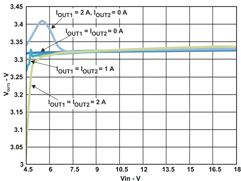
Figure 4-6. TPS54294EVM Converter 2 Line Regulation
