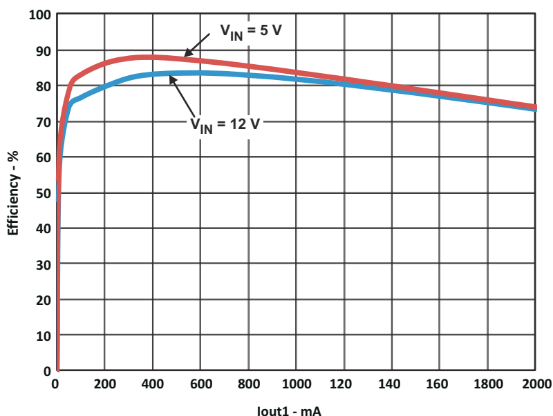
Figure 4-1. TPS54294EVM Converter 1 Efficiency
