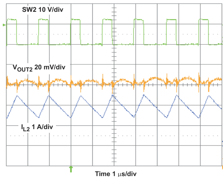
Figure 4-12. TPS54294EVM Converter 2 Output Voltage Ripple
