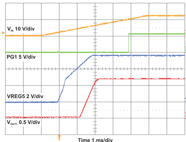
Figure 4-16. TPS54294EVM Converter 1 Start-Up Relative to V_{IN}
