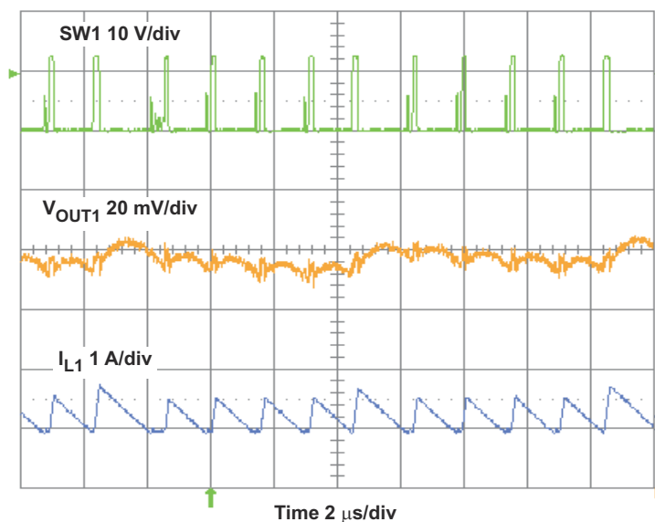
Figure 4-10. TPS54294EVM Converter 1 Eco-mode™ Output Voltage Ripple
