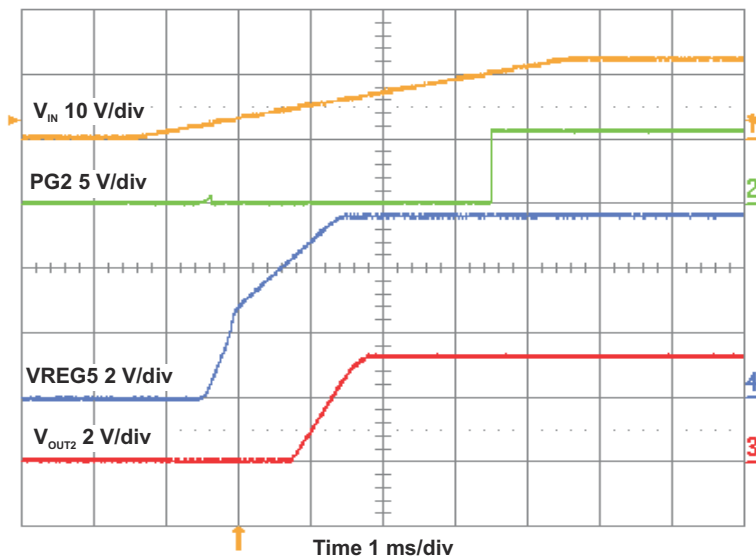
Figure 4-20. TPS54294EVM Converter 2 Start-Up Relative to V_{IN}
