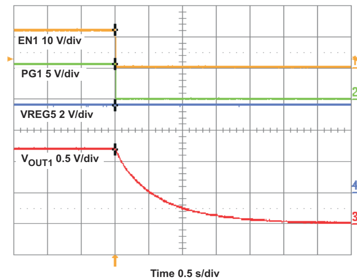
Figure 4-19. TPS54294EVM Shut-Down Relative to EN1
