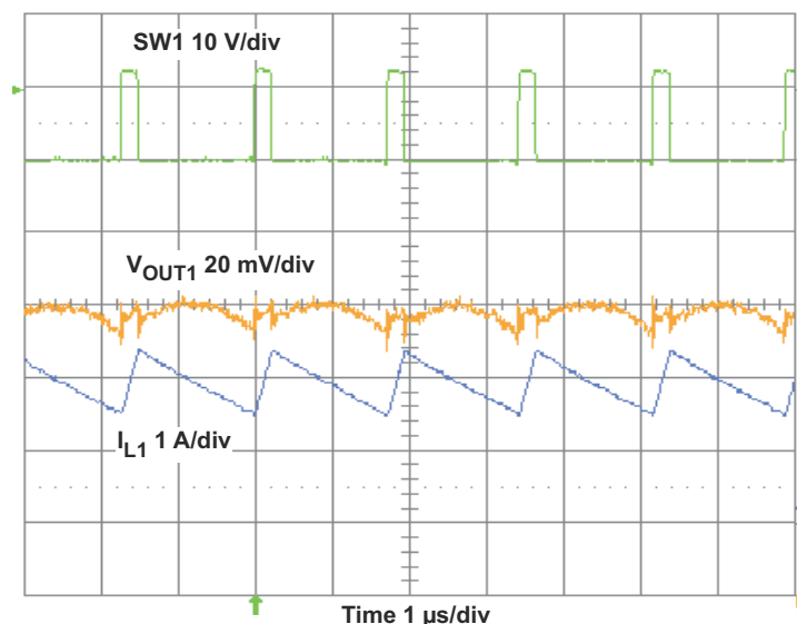
Figure 4-9. TPS54294EVM Converter 1 Output Voltage Ripple
