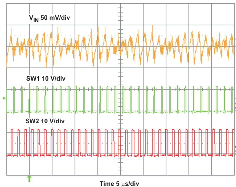
Figure 4-15. TPS54294EVM Input Voltage Ripple
