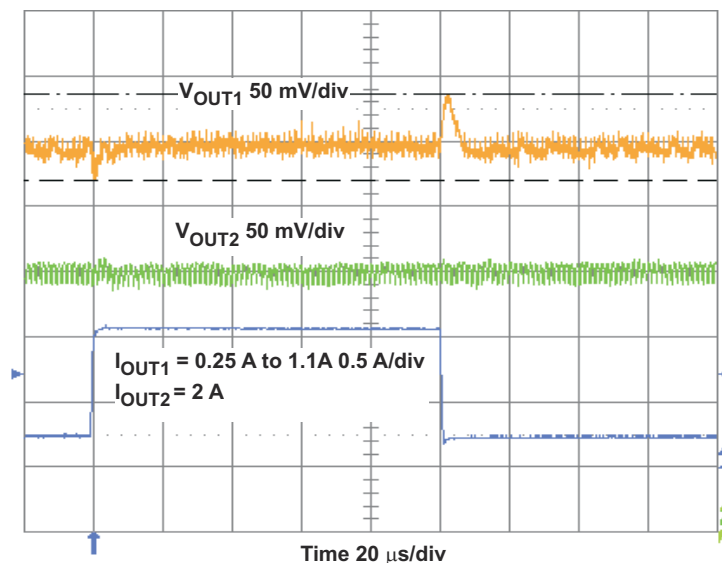
Figure 4-7. TPS54294EVM Converter 1 Load Transient Response
