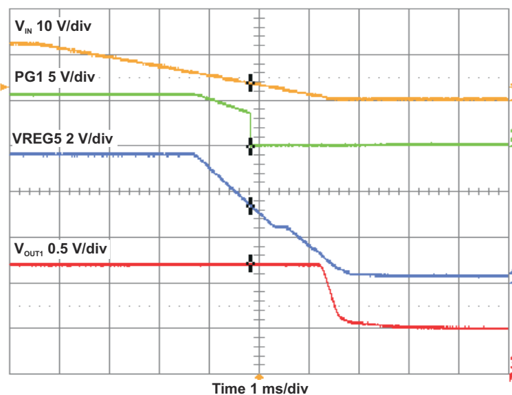
Figure 4-17. TPS54294EVM Converter 1 Shut-Down Relative to V_{IN}
