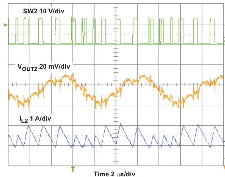
Figure 4-13. TPS54294EVM Converter 2 Eco-mode™ Output Voltage Ripple
