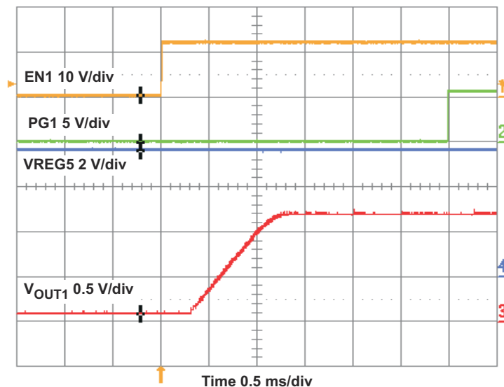
Figure 4-18. TPS54294EVM Start-Up Relative to EN1
