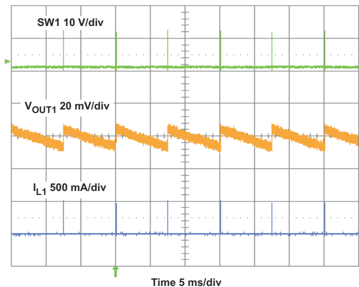
Figure 4-11. TPS54294EVM Converter 1 Eco-mode™ Output Voltage Ripple at No Load
