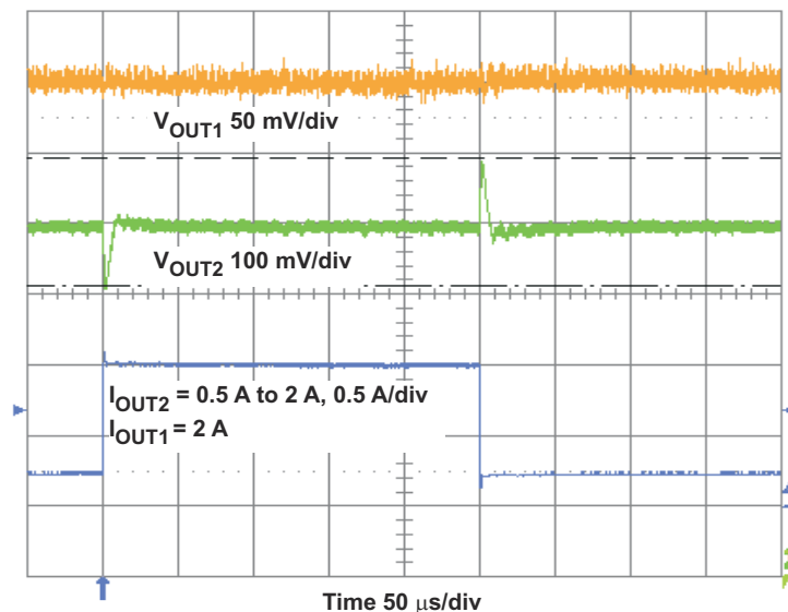
Figure 4-8. TPS54294EVM Converter 2 Load Transient Response
