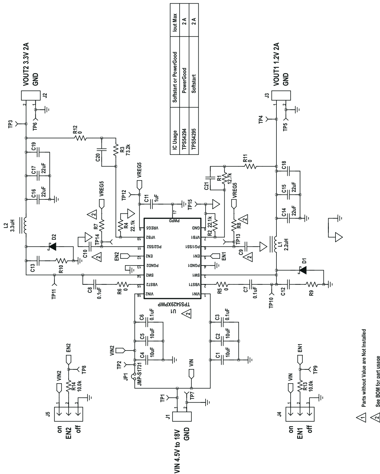
Figure 6-1. TPS54294EVM Schematic Diagram
