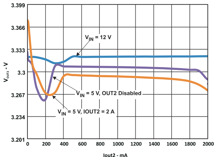
Figure 4-4. TPS54294EVM Converter 2 Load Regulation
