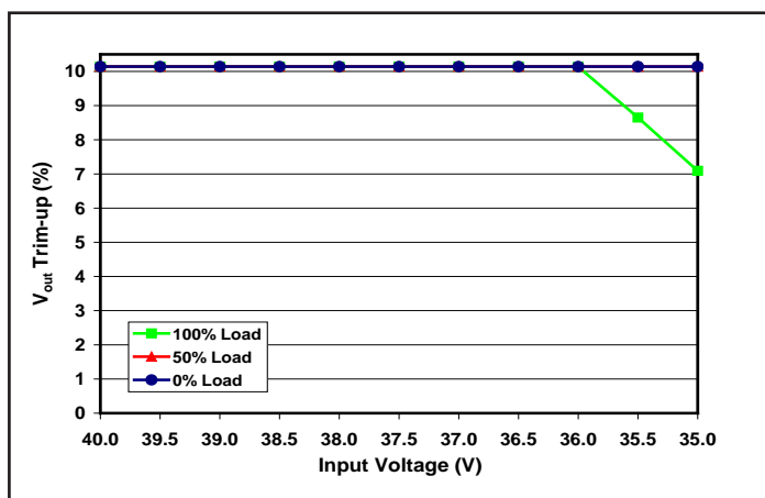
Figure 23: Achievable trim-up percentage vs. input voltage, at output loads of 0%, 50% and full load.
