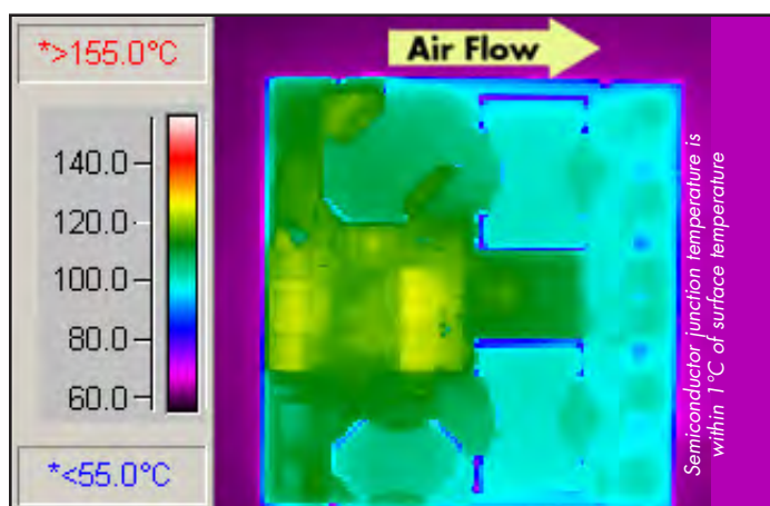
Figure 6: Thermal plot of converter at 18 amp load current (217 Watts) with 55°C air flowing at the rate of 200 LFM. Air is flowing across the converter from input to output (nominal input voltage).
