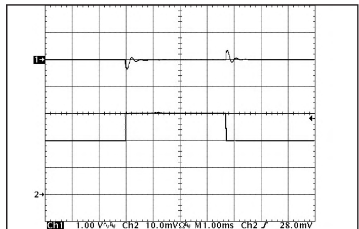
Figure 12: Output voltage response to step-change in load current (50%-75%-50% of I_{out(max)} ; dI/dt = 5A/\mu s ). Load cap: 480 \mu F , 15 m \Omega ESR tantalum and 1 \mu F ceramic. Top trace: V_{out} (1V/div), Bottom trace: I_{out} (5A/div).
