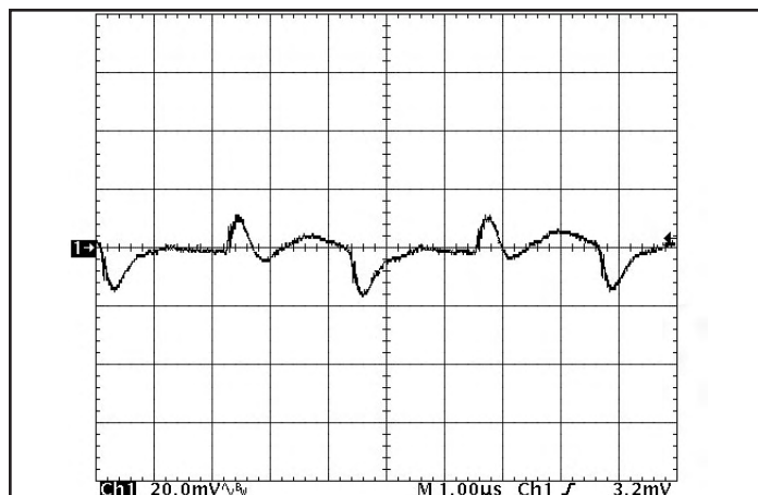
Figure 16: Output Voltage Ripple at nominal input voltage and rated load current (20 mV/div). Load capacitance: 1\ \mu\text{F} ceramic capacitor and 15\ \mu\text{F} tantalum capacitor. Bandwidth: 20 MHz. (See Figure 13)
