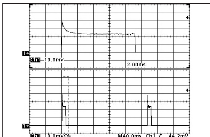
Figure 18: Load current (10A/div) as a function of time when the converter attempts to turn on into a 1\ \text{m}\Omega short circuit. Top trace (2ms/div) is an expansion of the on-time portion of the bottom trace.
