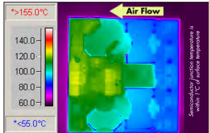
Figure 8: Thermal plot of converter at 17 amp load current (204 Watts) with 55°C air flowing at the rate of 200 LFM. Air is flowing across the converter from output to input (nominal input voltage).
