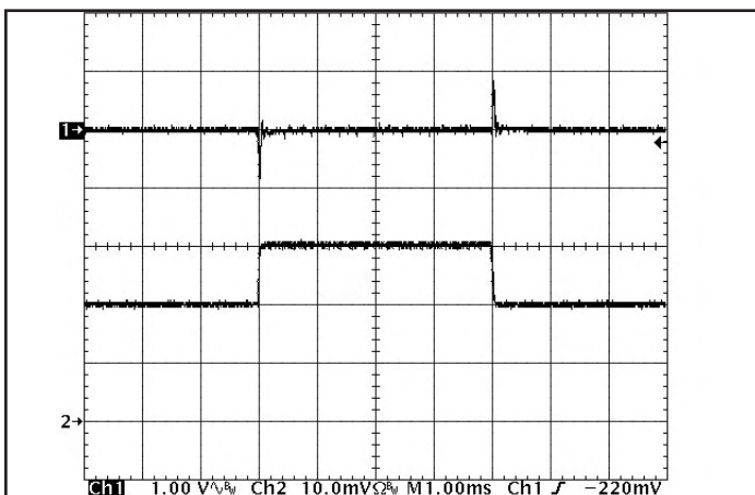
Figure 11: Output voltage response to step-change in load current (50%-75%-50% of I_{out(max)} ; dI/dt = 0.1A/\mu s ). Load cap: 15 \mu F , 450 mW ESR tantalum and 1 \mu F ceramic. Top trace: V_{out} (1V/div), Bottom trace: I_{out} (5A/div).
