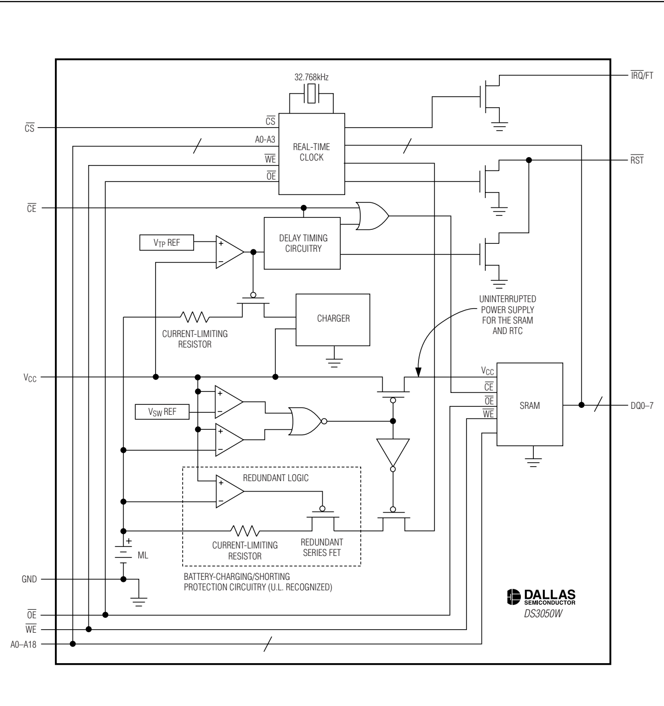
Functional Diagram
