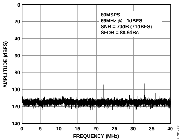
Figure 8. Single-Tone FFT with f_{IN} = 69 MHz
