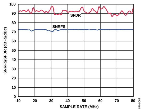
Figure 14. SNR/SFDR vs. Sample Rate with AIN = 9.7 MHz
