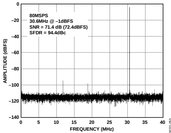
Figure 7. Single-Tone FFT with f_{IN} = 30.6 MHz
