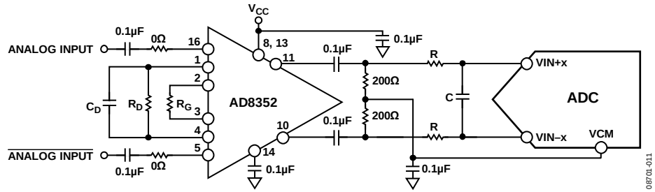
Figure 32. Differential Input Configuration Using the AD8352
