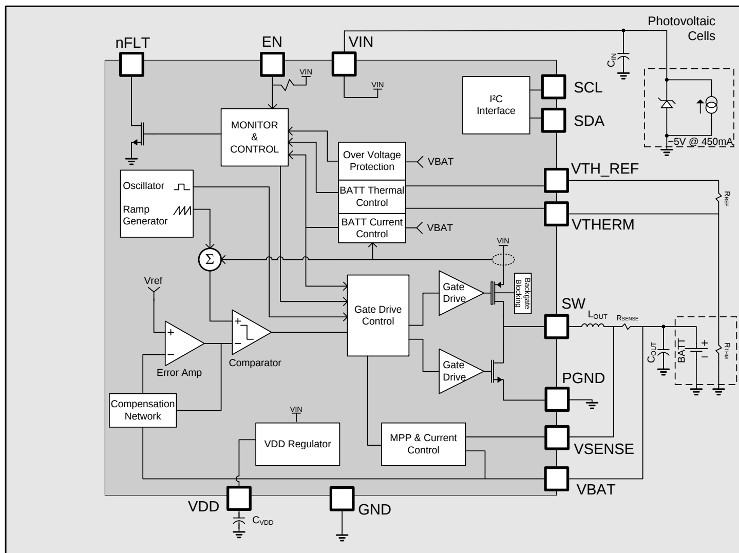
Figure 2: TS52001 Block Diagram
