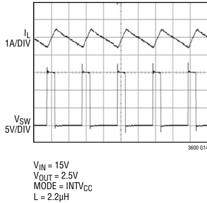
Continuous Conduction Mode Operation
