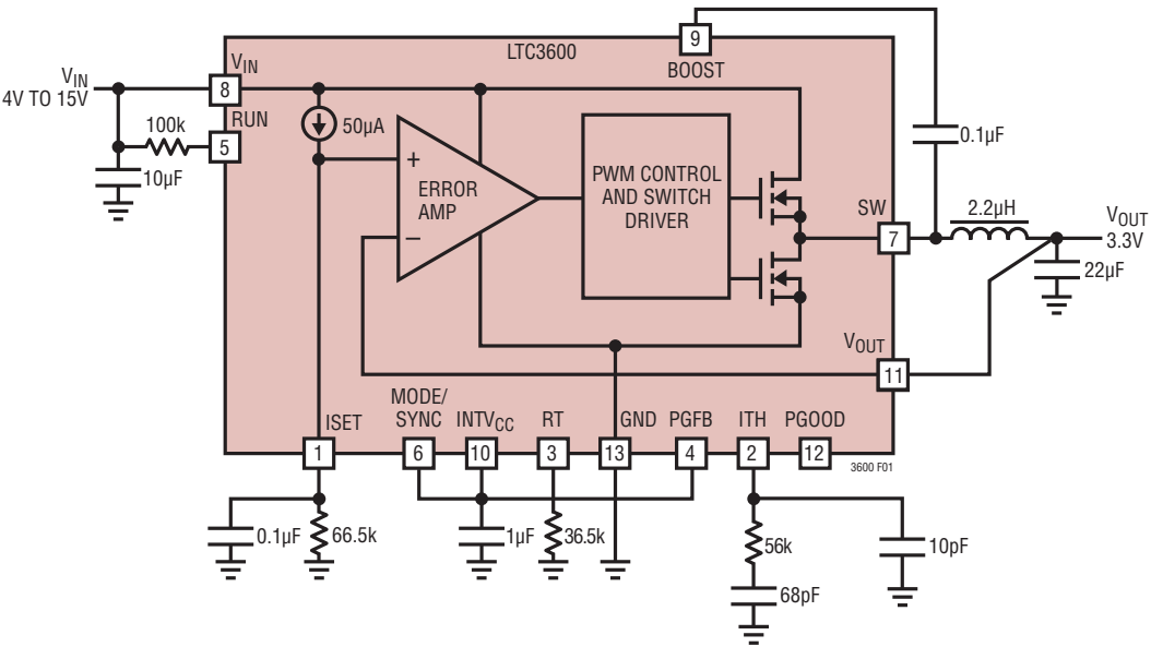
Figure 1. 12V to 3.3V 1MHz Buck Regulator
