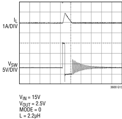
Discontinuous Conduction Mode Operation
