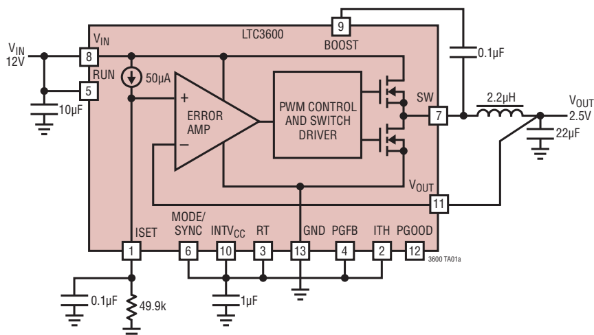
High Efficiency, 1MHz, 1.5A Step-Down Converter
