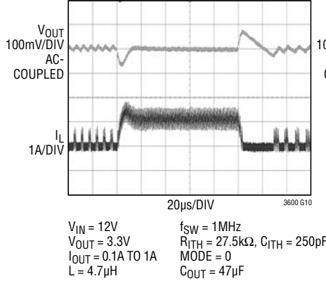
Transient Response DCM, Operation, External Compensation
