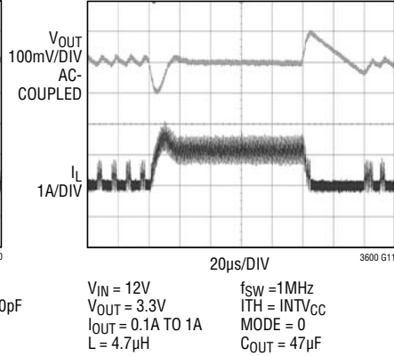
Transient Response DCM, Operation, Internal Compensation
