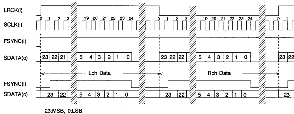
Figure 1. Serial Data Timing (Slave mode)
