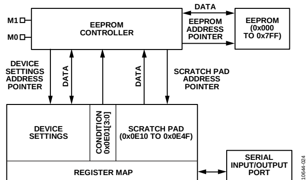
Figure 43. EEPROM Functional Diagram
