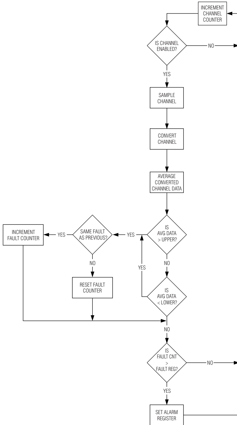
Figure 4. Alarm Flowchart
