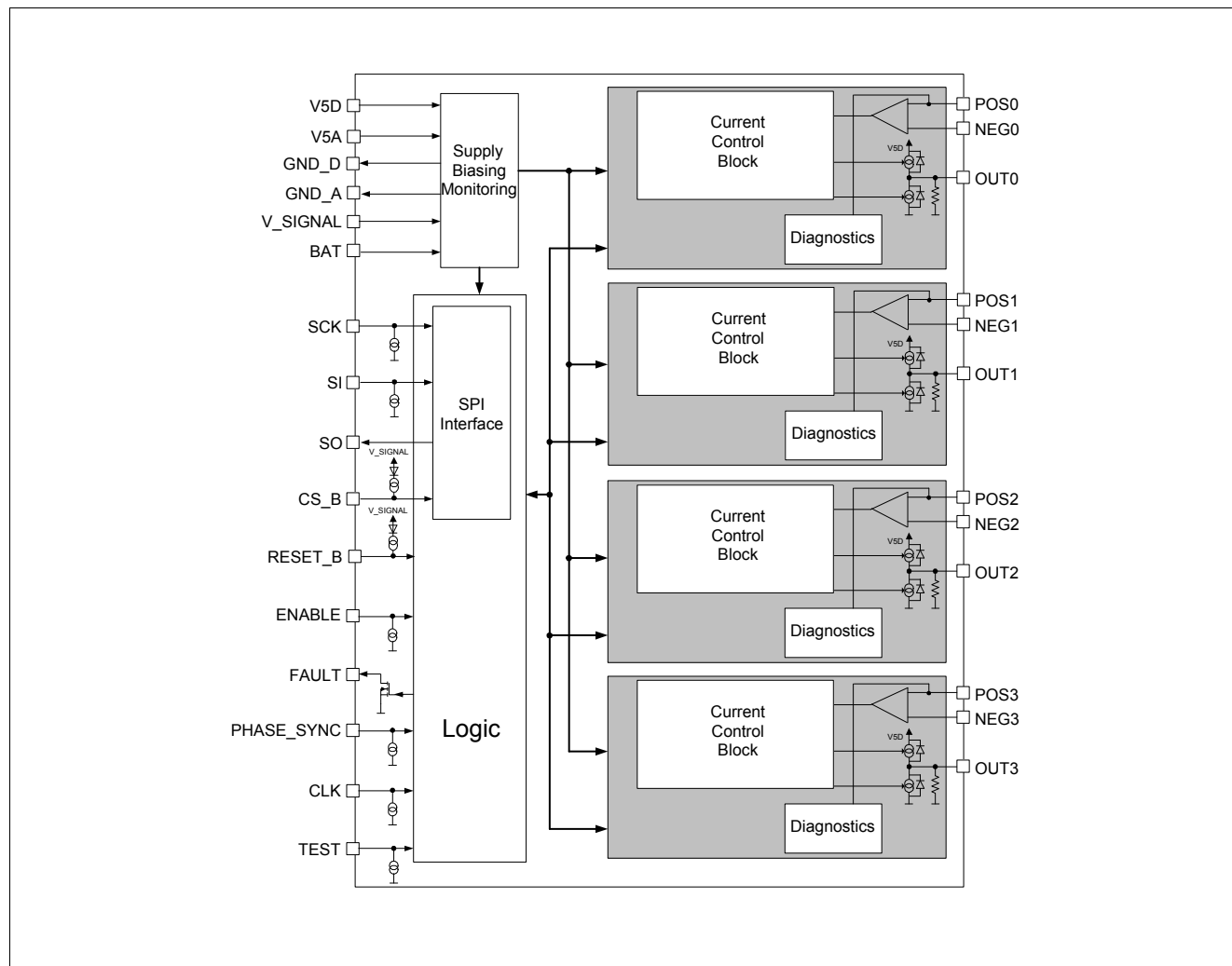
Figure 7 Block Diagram
