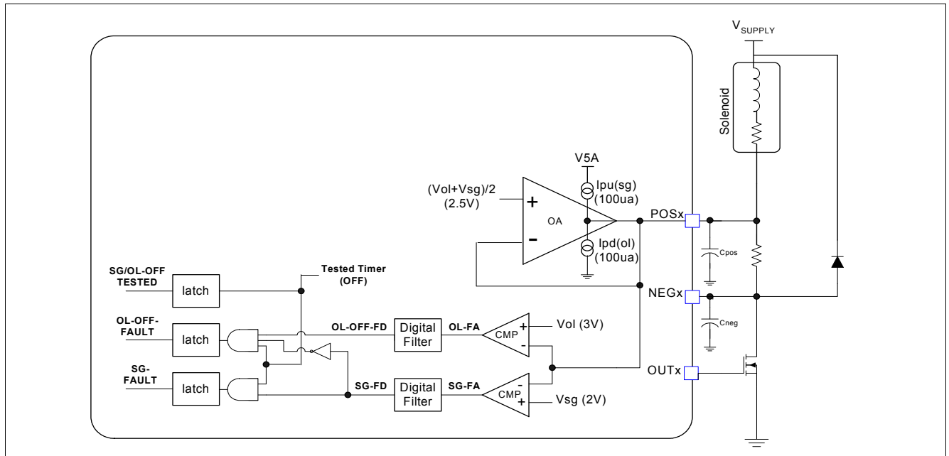
Figure 14 Off-State Diagnostics
