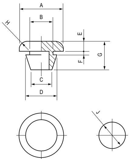
取付穴図 Hole for Installation
