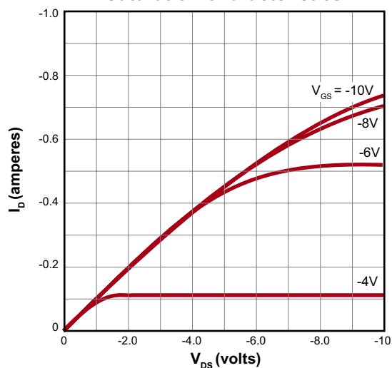
Saturation Characteristics
