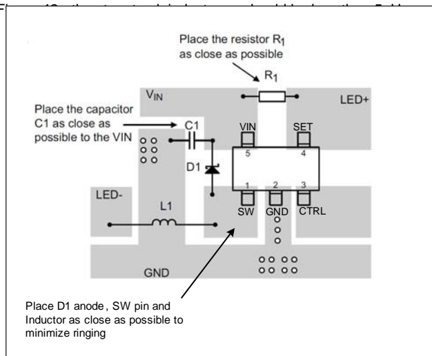
Figure 42 Recommended PCB Layout
