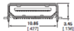
HDMI-C Connector
